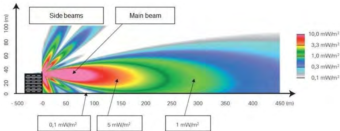
Vertically focused beam pattern of a sector antenna
